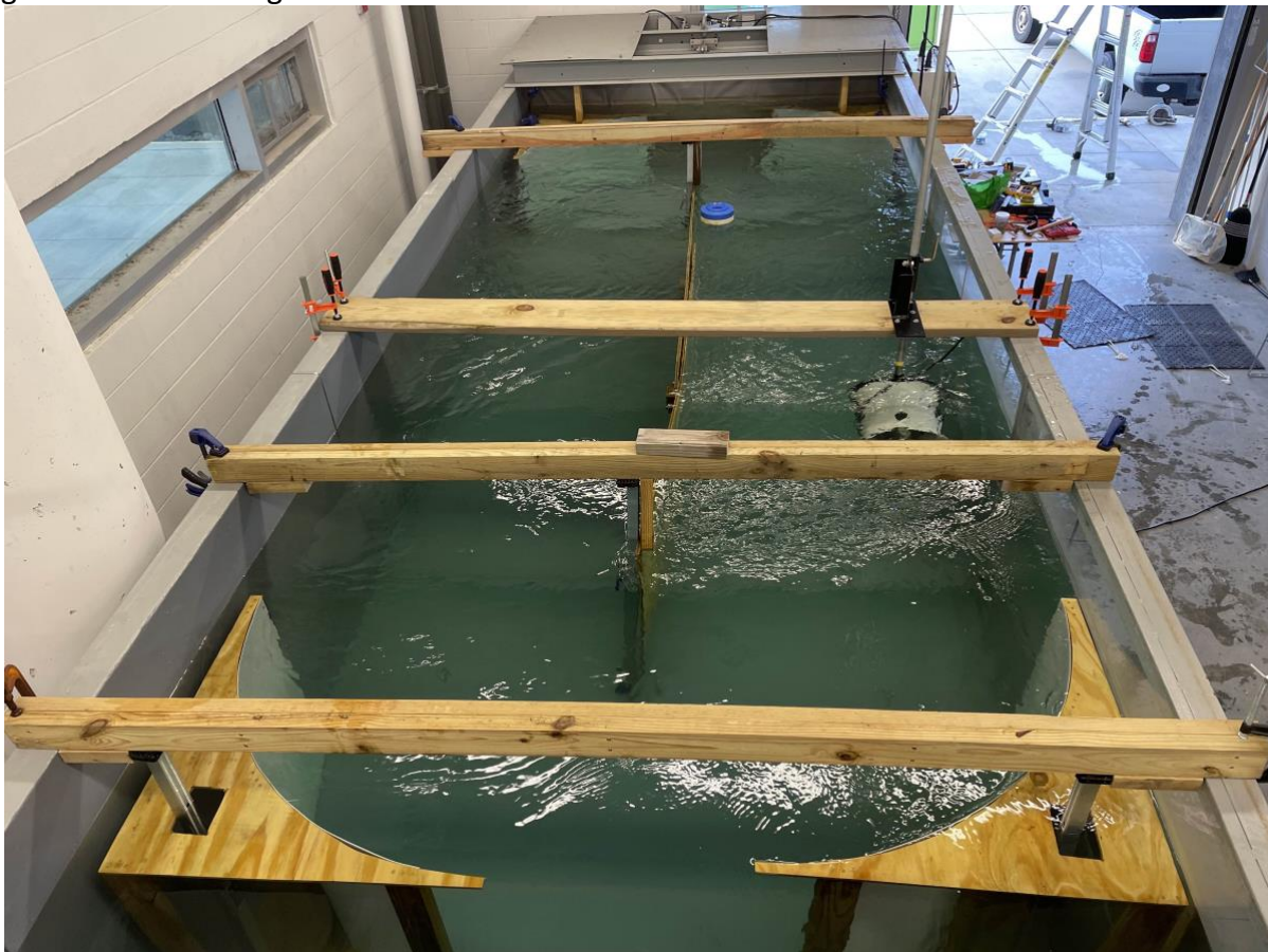
Figure 3: Recirculating flume tank
