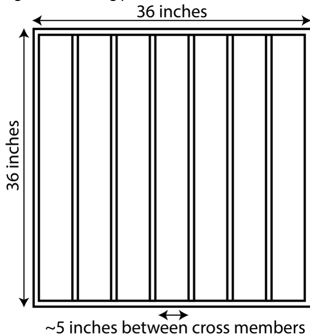
Figure 2: Mooring platform
